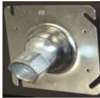
Galvanized steel Thread 3/4" Weight limit 75lbs
