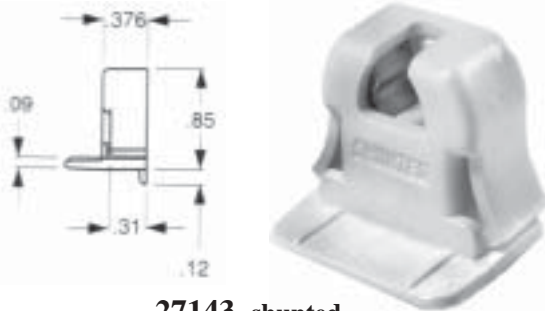
27143 -shunted Cutout size: .376 x .772
