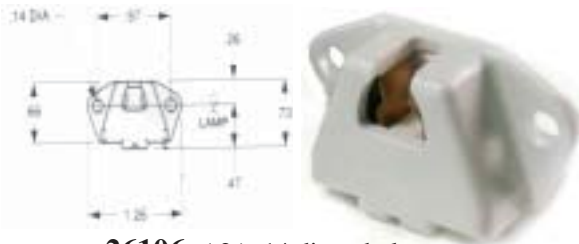
26106 -( 2 ) .14 diam. holes Mounting holes .97 C to °C
