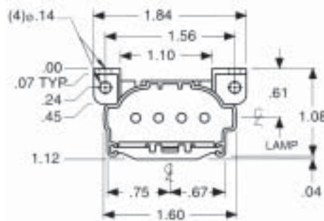
Screw Down Circline
