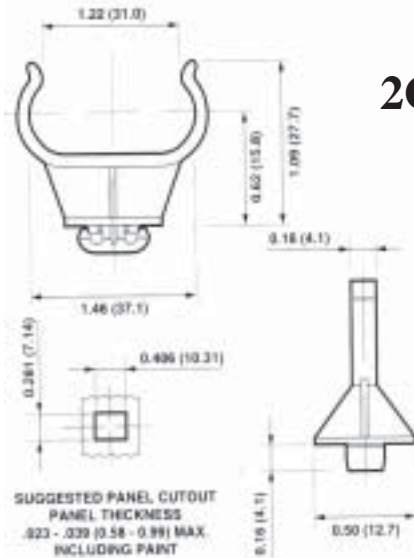
25611 -2G11 plastic support
